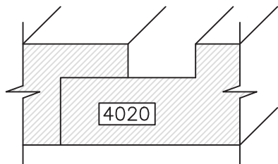
1/2" \times 1/4" Gap
