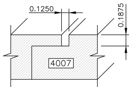
1/8"x3/16" Gap
