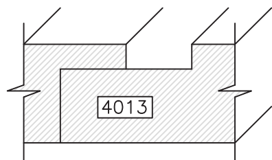
1/2"x3/16" Gap
