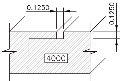
1/8" \times 1/8" Gap
