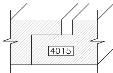
3/16" \times 1/4" Gap
