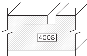
3/16"x3/16" Gap
