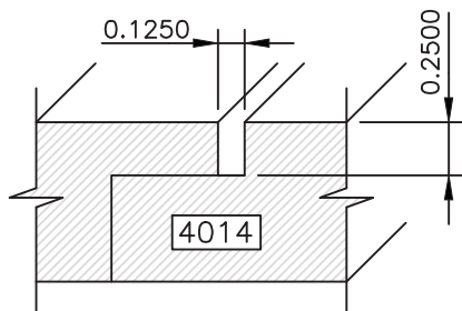
1/8" \times 1/4" Gap
